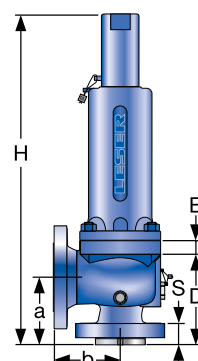
Conventional design
