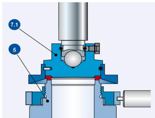
Figure 9.5.3.2-1: Stellited sealing surfaces
